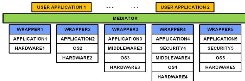
Figure 22 SeNsIM Architecture
