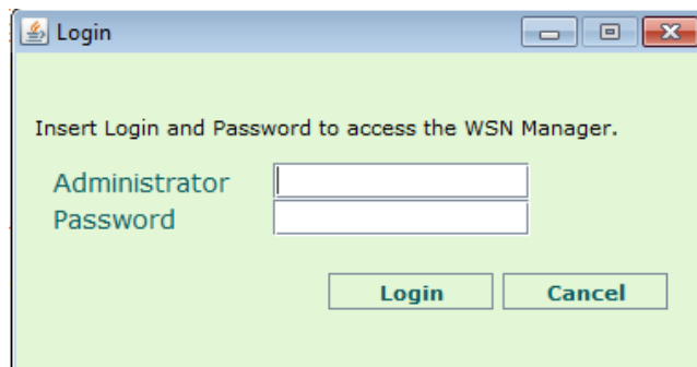
Figure 24 Login Panel
