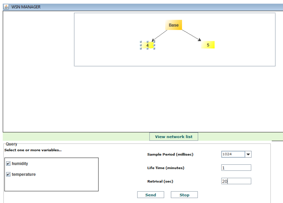
Figure 27 Manager Panel
